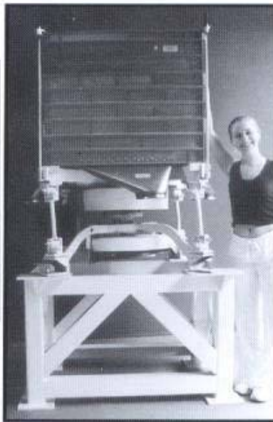
7 deck multiple separation gyratory sifter
